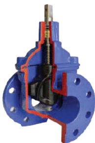
Mono Design Gate Valve
